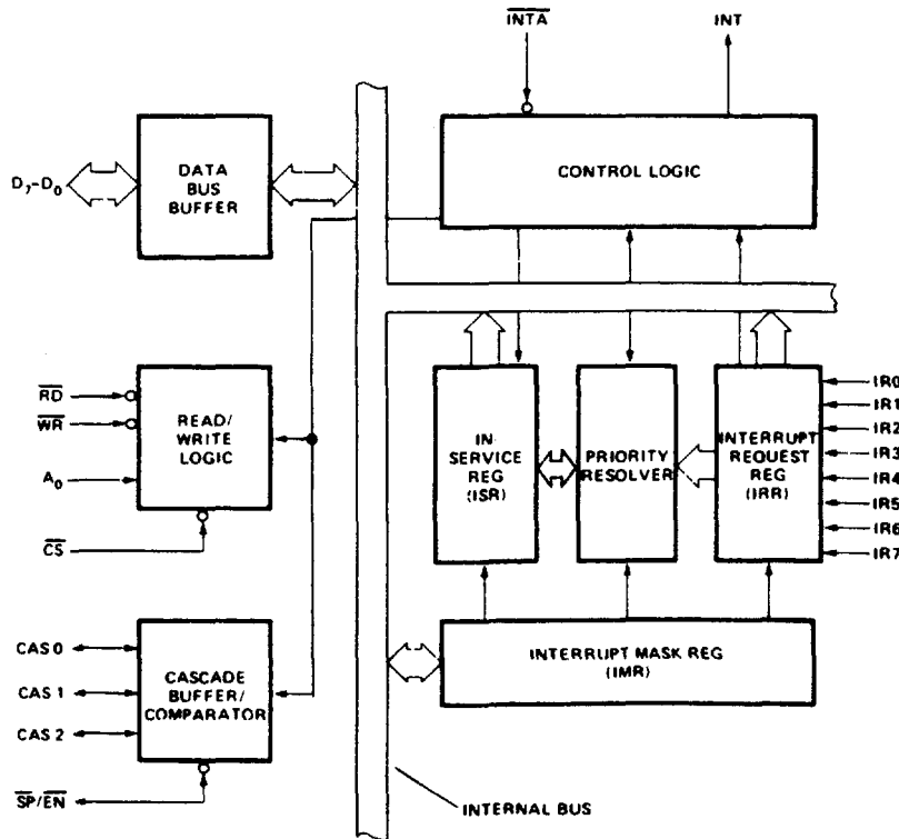
8259 BLOCK DIAGRAM
