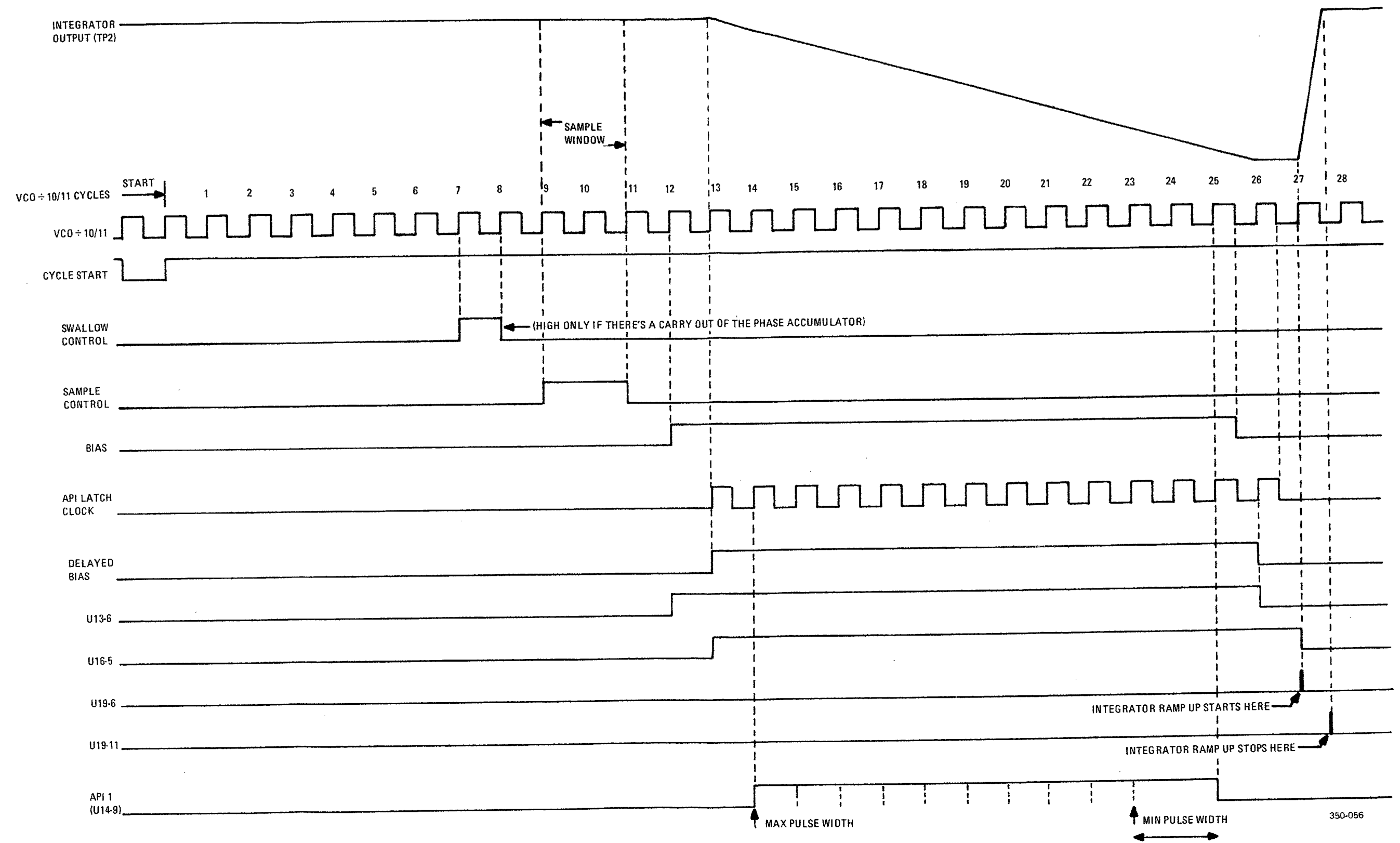
Figure FO-7. Synthesizer Integrator Timing Diagram.
