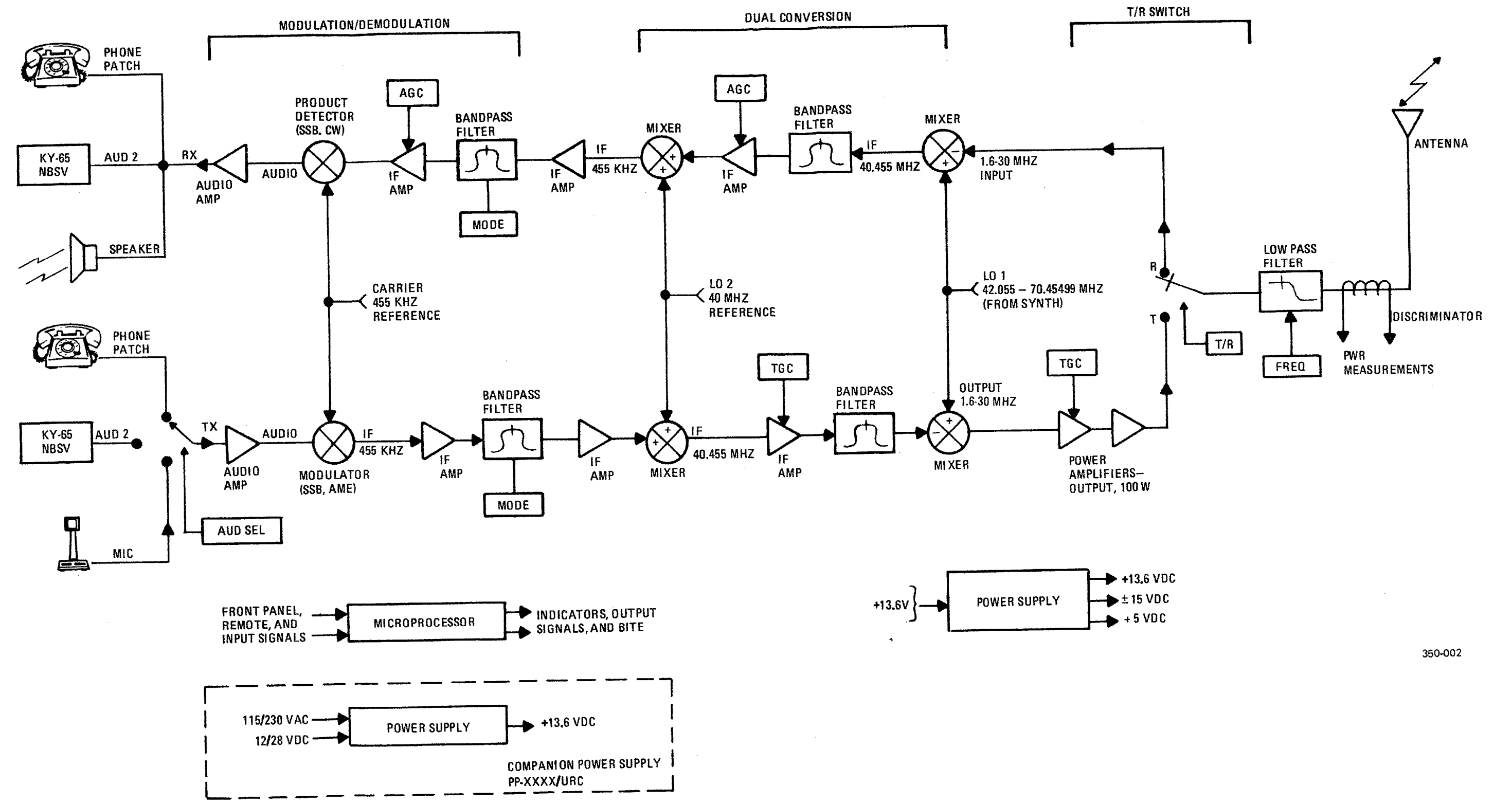
Figure FO-13. Simplified Functional Diagram, 100 Watt Transceiver
